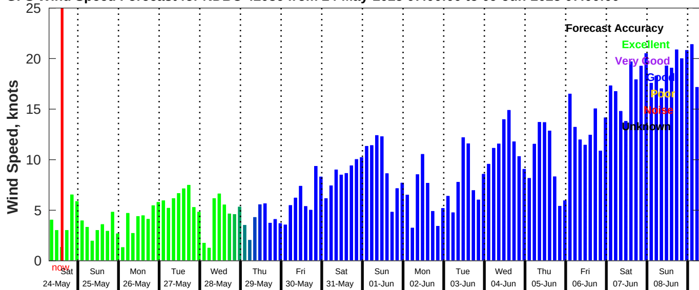
GFS Wind Speed Forecast for NDBC 42036 from 24-May-2025 07:00:00 to 09-Jun-2025 07:00:00
