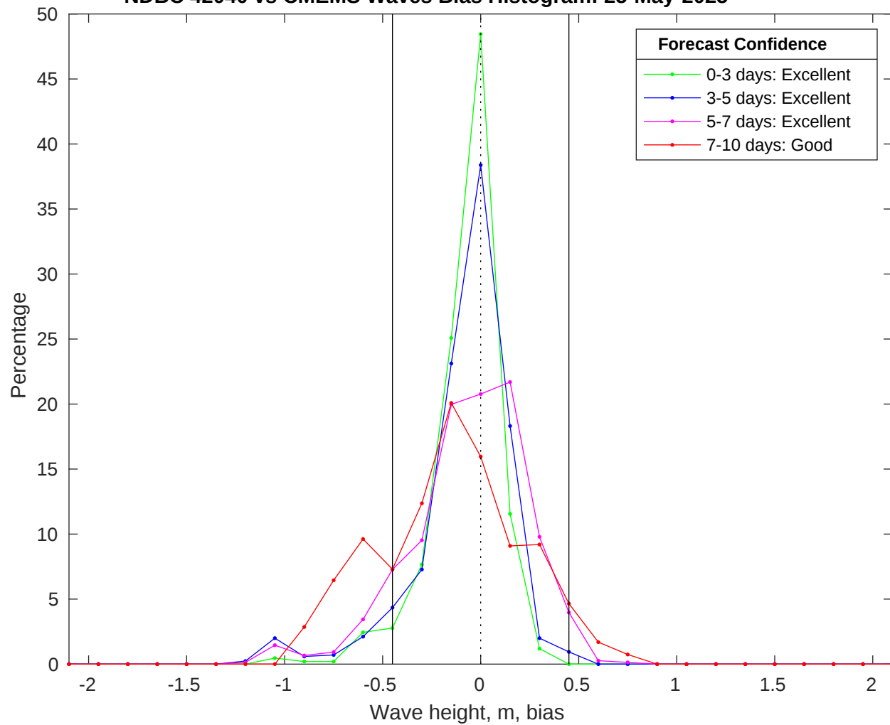
NDBC 42040 vs CMEMS Waves Bias Histogram: 25-May-2025
