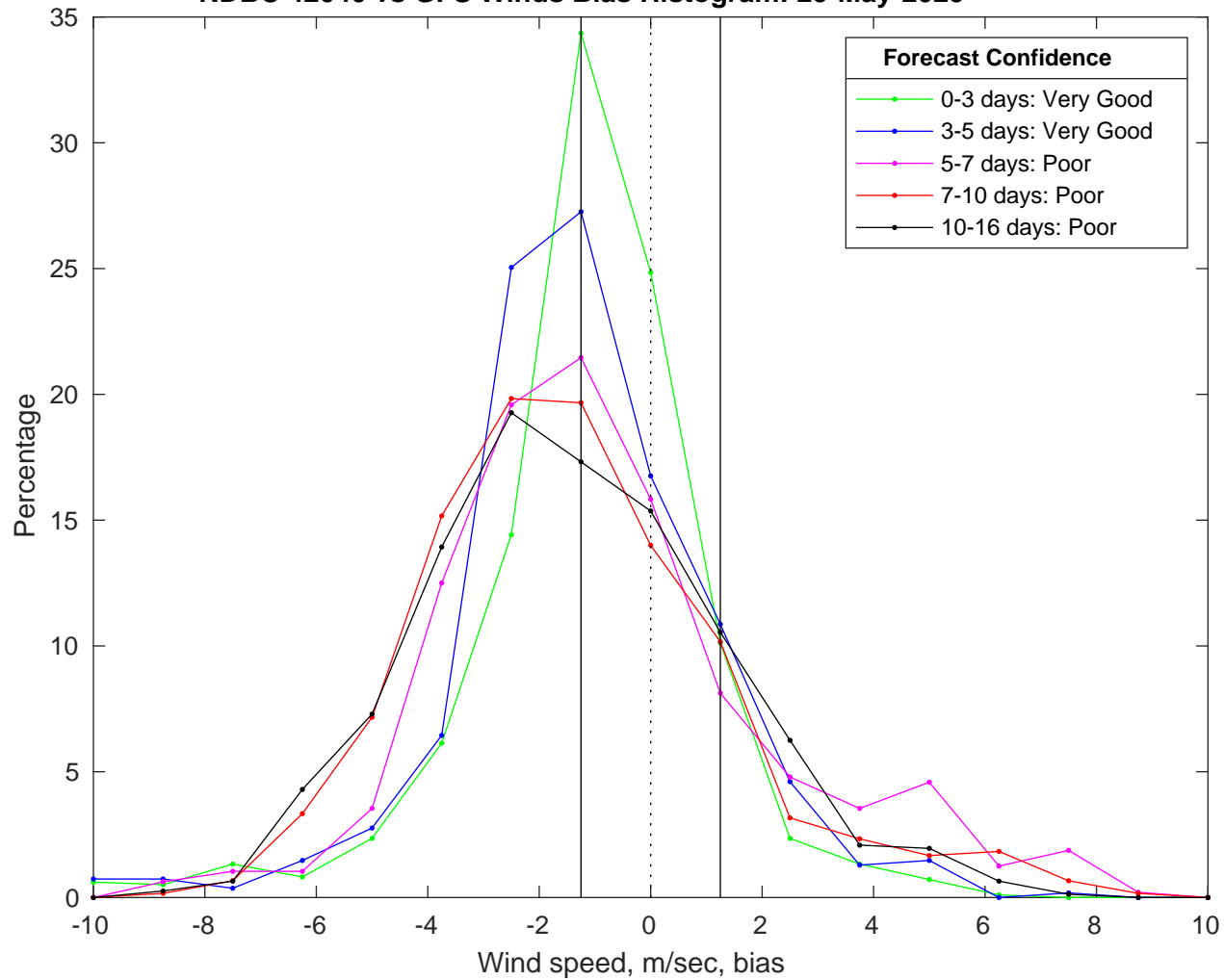
NDBC 42040 vs GFS Winds Bias Histogram: 25-May-2025
