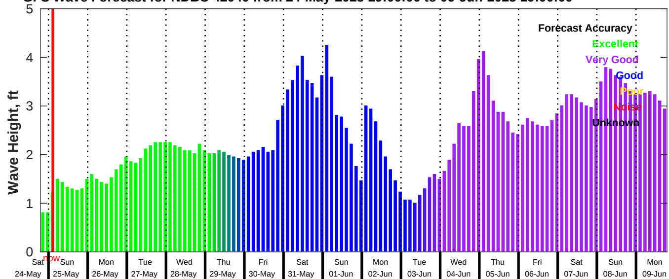
GFS Wave Forecast for NDBC 42040 from 24-May-2025 19:00:00 to 09-Jun-2025 19:00:00
