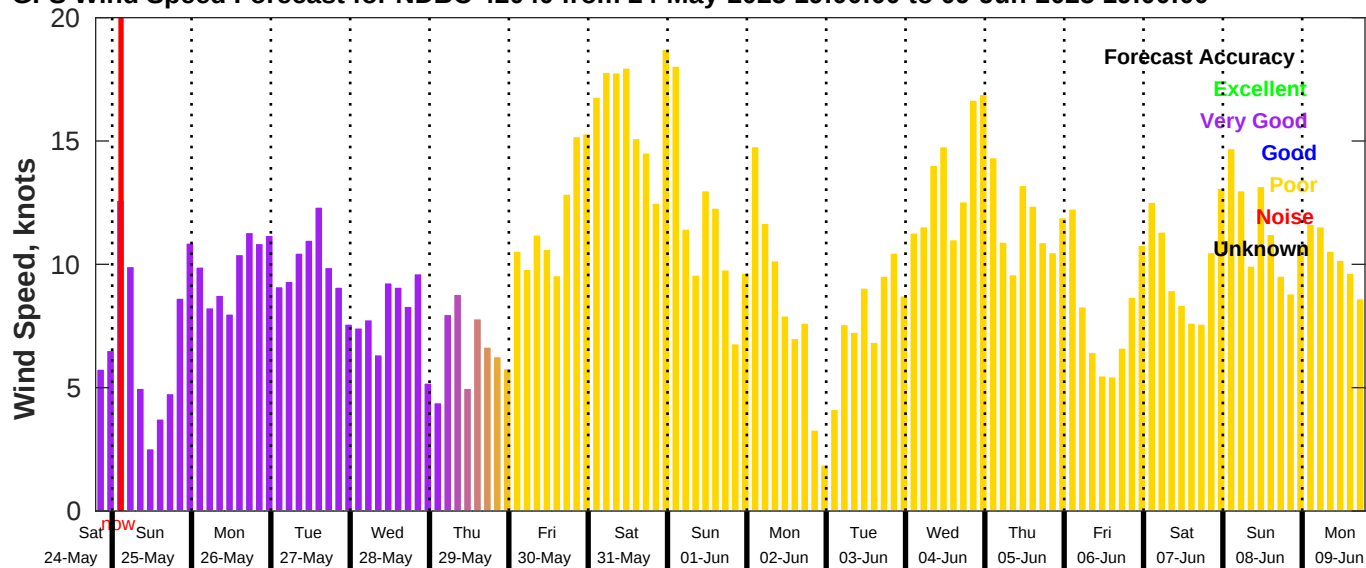
GFS Wind Speed Forecast for NDBC 42040 from 24-May-2025 19:00:00 to 09-Jun-2025 19:00:00
