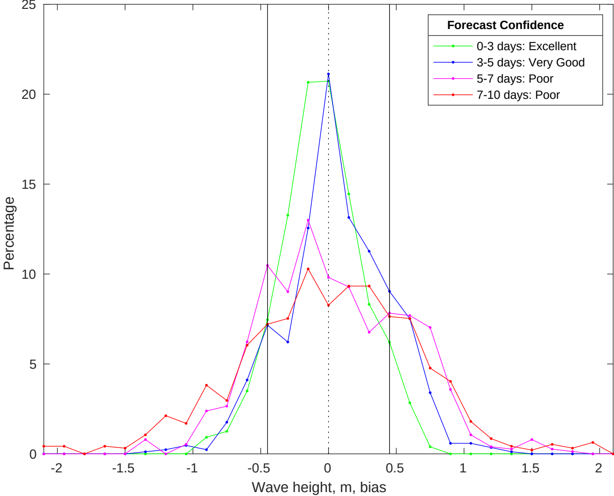
NDBC 46011 vs CMEMS Waves Bias Histogram: 25-May-2025
