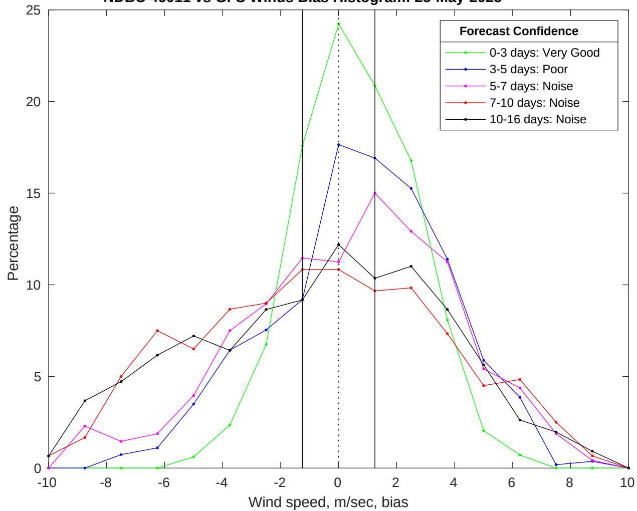
NDBC 46011 vs GFS Winds Bias Histogram: 25-May-2025
