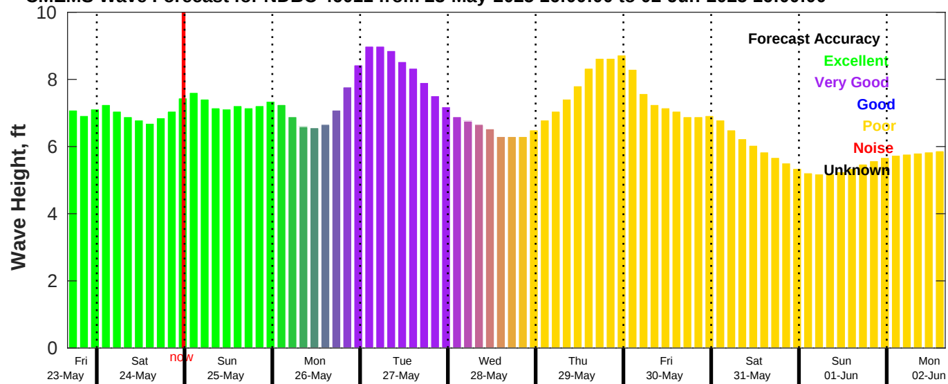
CMEMS Wave Forecast for NDBC 46011 from 23-May-2025 16:00:00 to 02-Jun-2025 16:00:00
