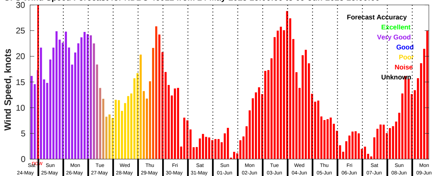
GFS Wind Speed Forecast for NDBC 46011 from 24-May-2025 16:00:00 to 09-Jun-2025 16:00:00
