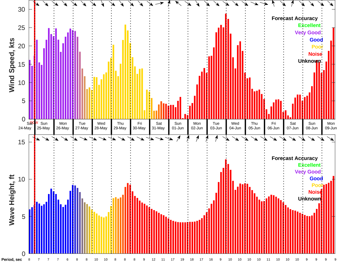
Wind & Wave Forecast for NDBC 46011 from 24-May-2025 16:00:00 to 09-Jun-2025 16:00:00
