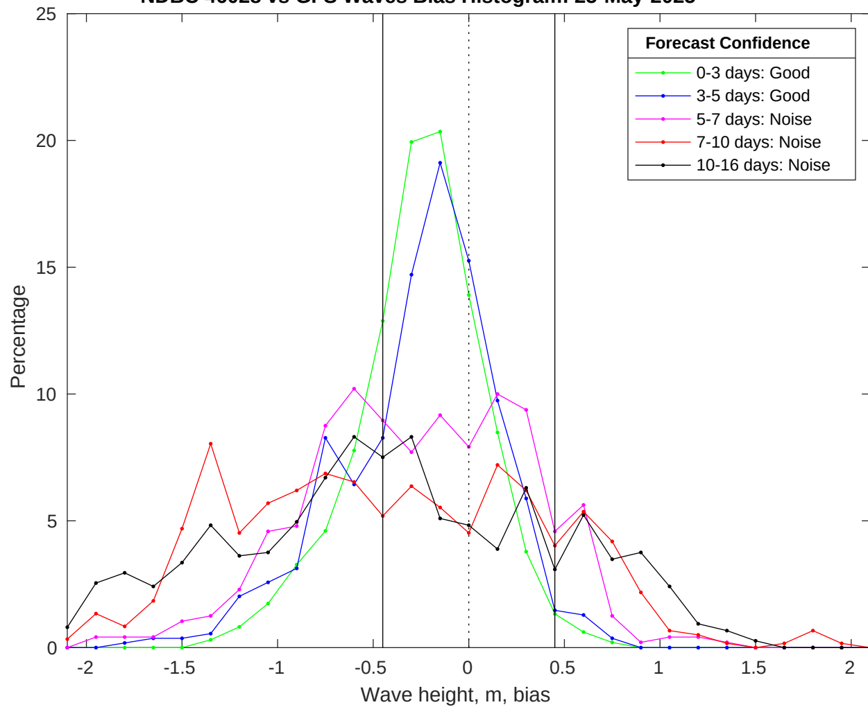
NDBC 46028 vs GFS Waves Bias Histogram: 25-May-2025
