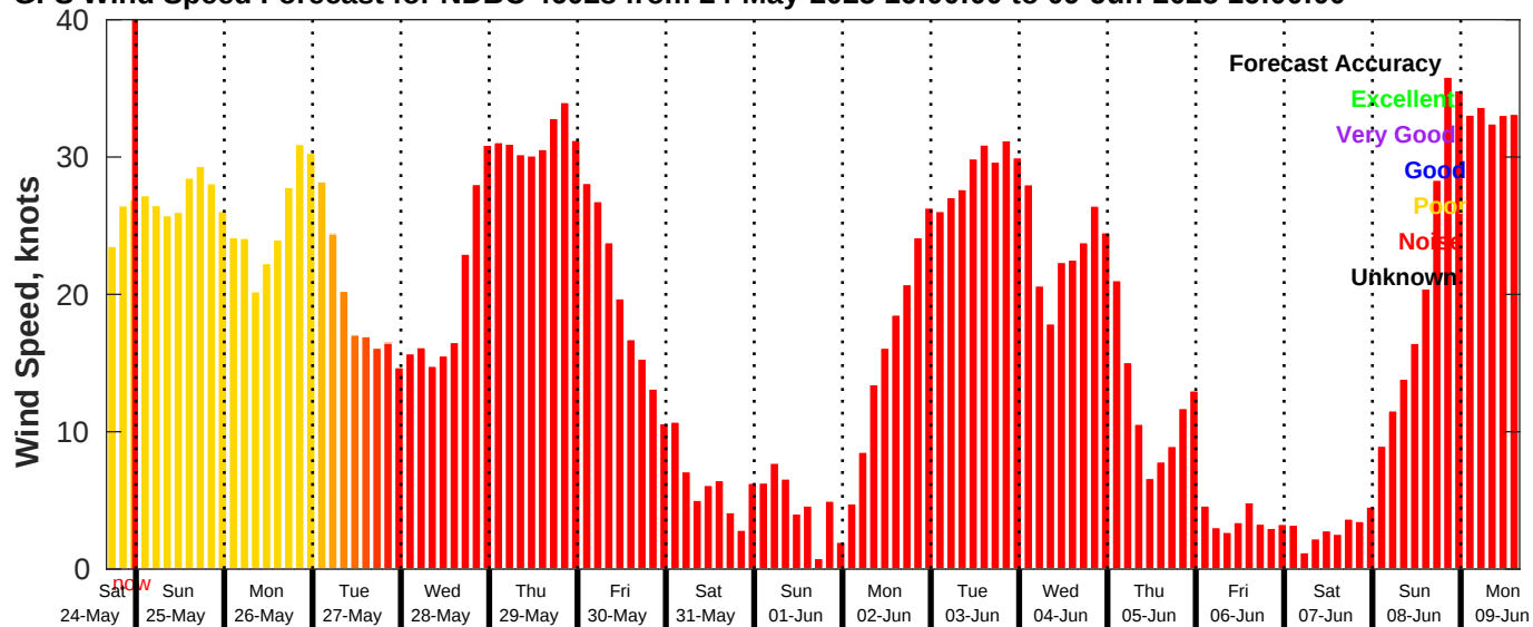
GFS Wind Speed Forecast for NDBC 46028 from 24-May-2025 16:00:00 to 09-Jun-2025 16:00:00
