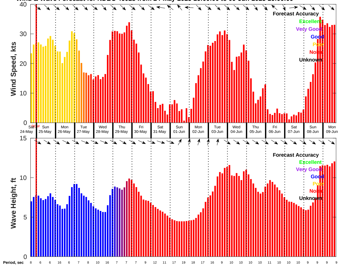
Wind & Wave Forecast for NDBC 46028 from 24-May-2025 16:00:00 to 09-Jun-2025 16:00:00
