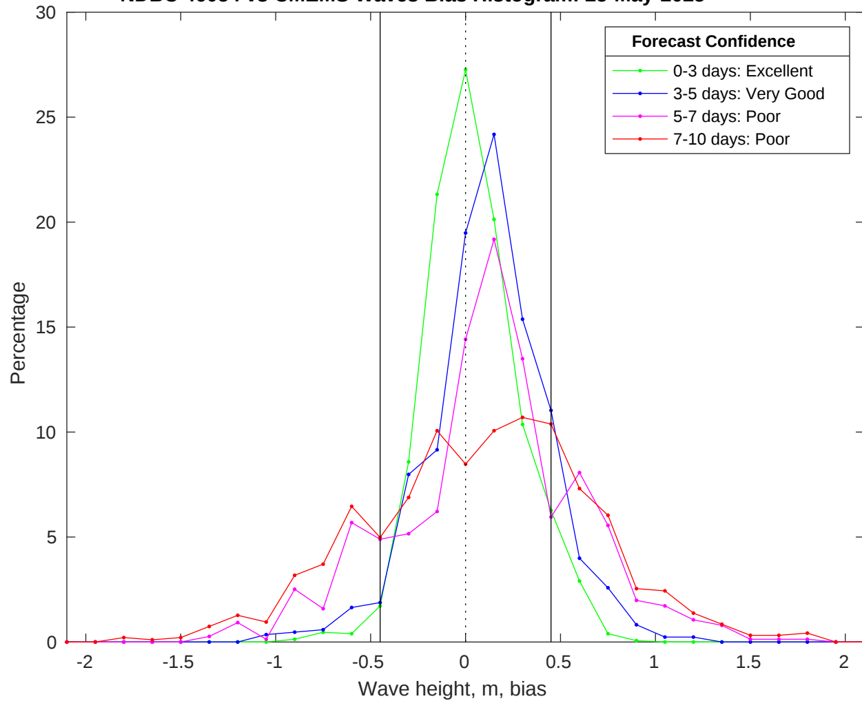
NDBC 46054 vs CMEMS Waves Bias Histogram: 25-May-2025
