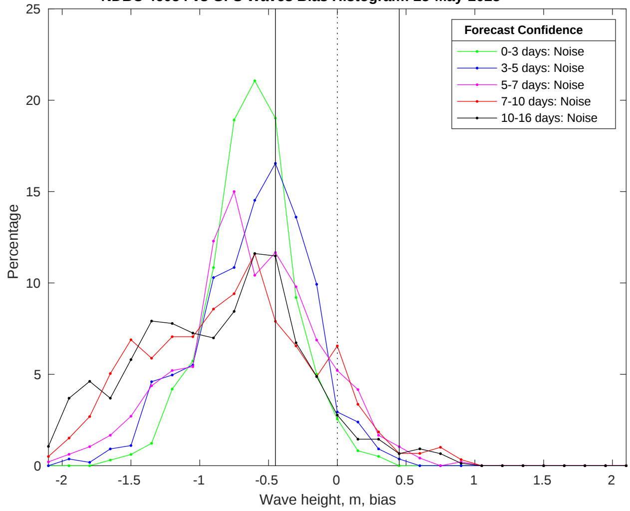
NDBC 46054 vs GFS Waves Bias Histogram: 25-May-2025
