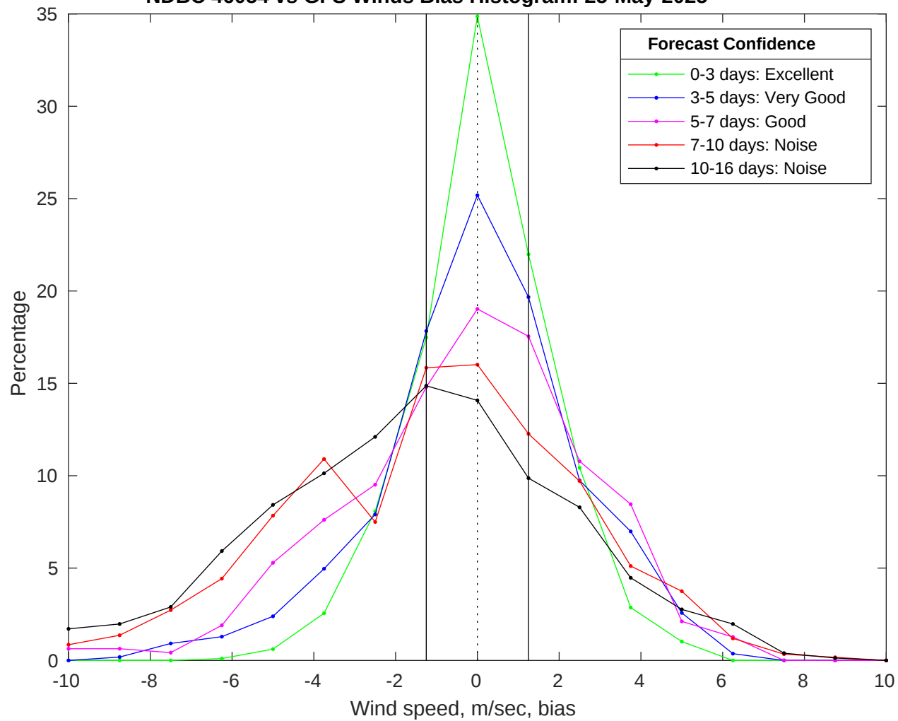
NDBC 46054 vs GFS Winds Bias Histogram: 25-May-2025
