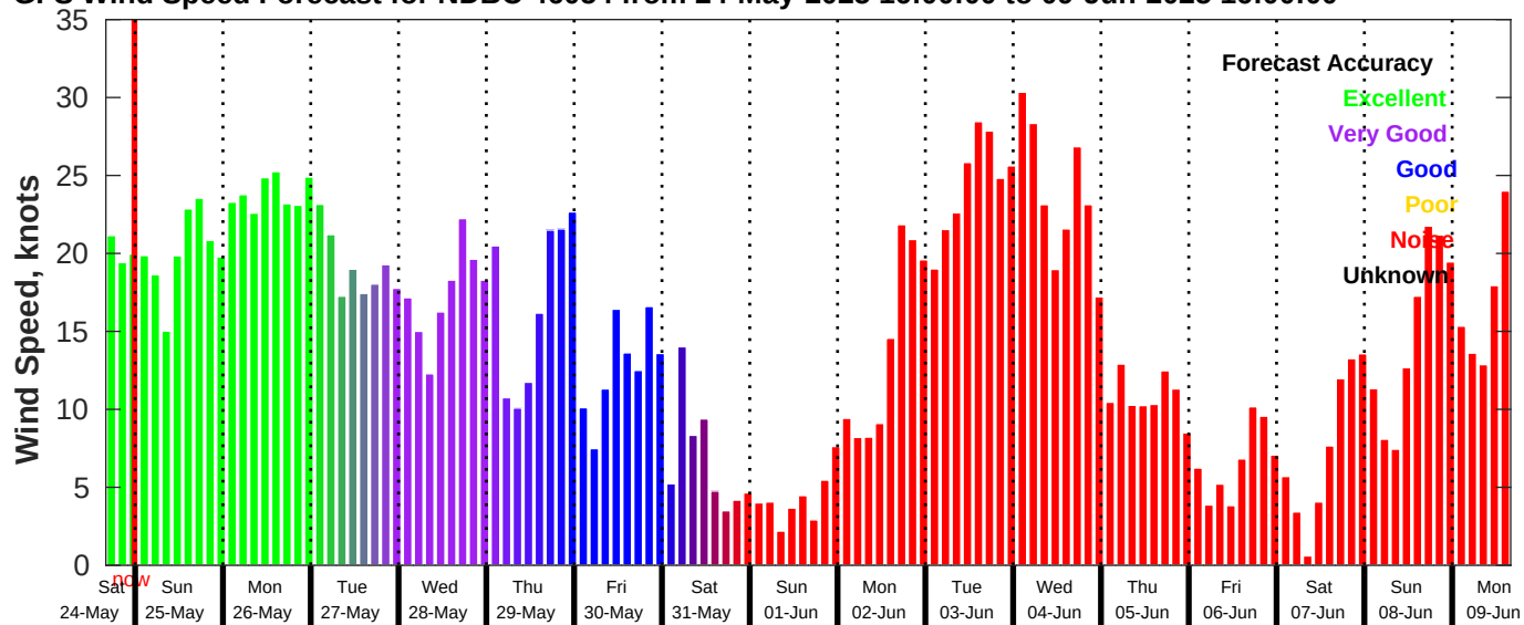
GFS Wind Speed Forecast for NDBC 46054 from 24-May-2025 16:00:00 to 09-Jun-2025 16:00:00
