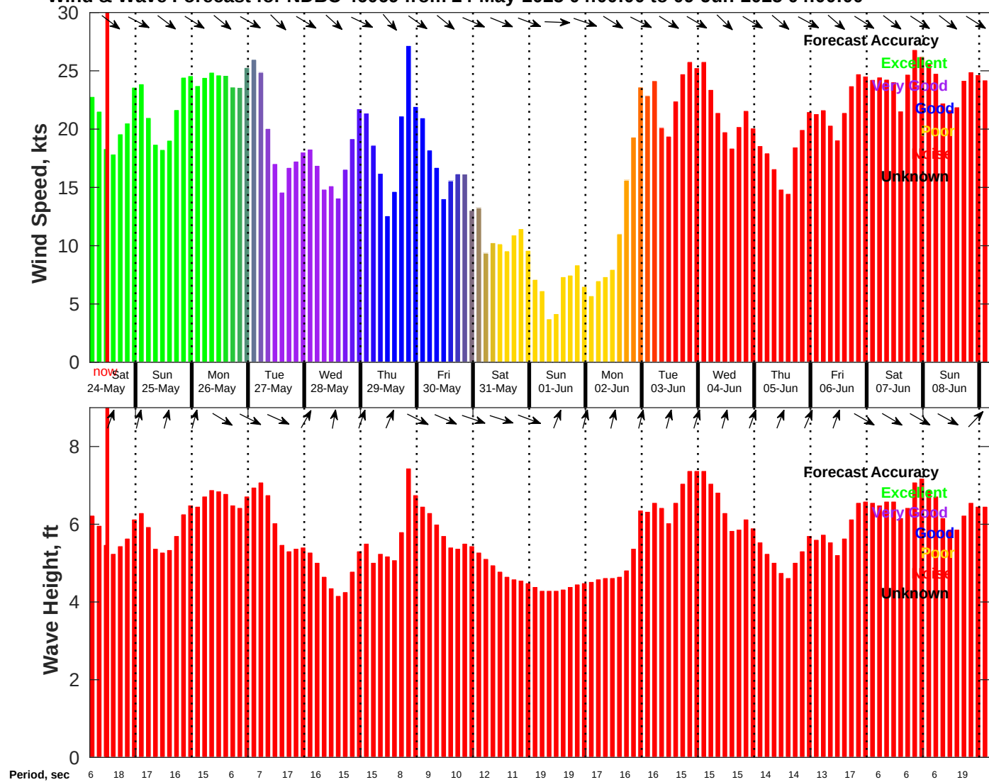
Wind & Wave Forecast for NDBC 46069 from 24-May-2025 04:00:00 to 09-Jun-2025 04:00:00
