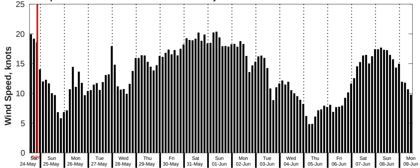
GFS Wind Speed Forecast for NDBC 51209 from 24-May-2025 13:00:00 to 09-Jun-2025 13:00:00
