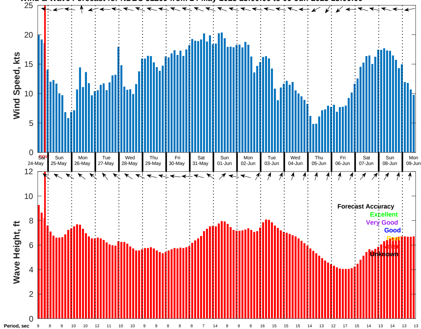
Wind & Wave Forecast for NDBC 51209 from 24-May-2025 13:00:00 to 09-Jun-2025 13:00:00
