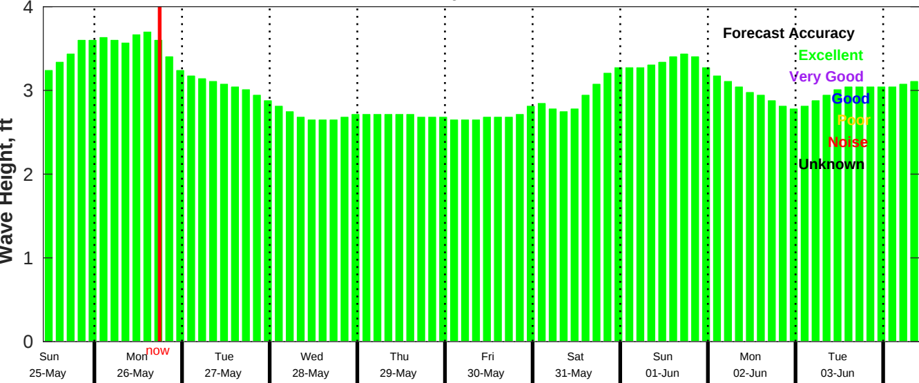
CMEMS Wave Forecast for NDBC 52211 from 24-May-2025 10:00:00 to 03-Jun-2025 10:00:00
