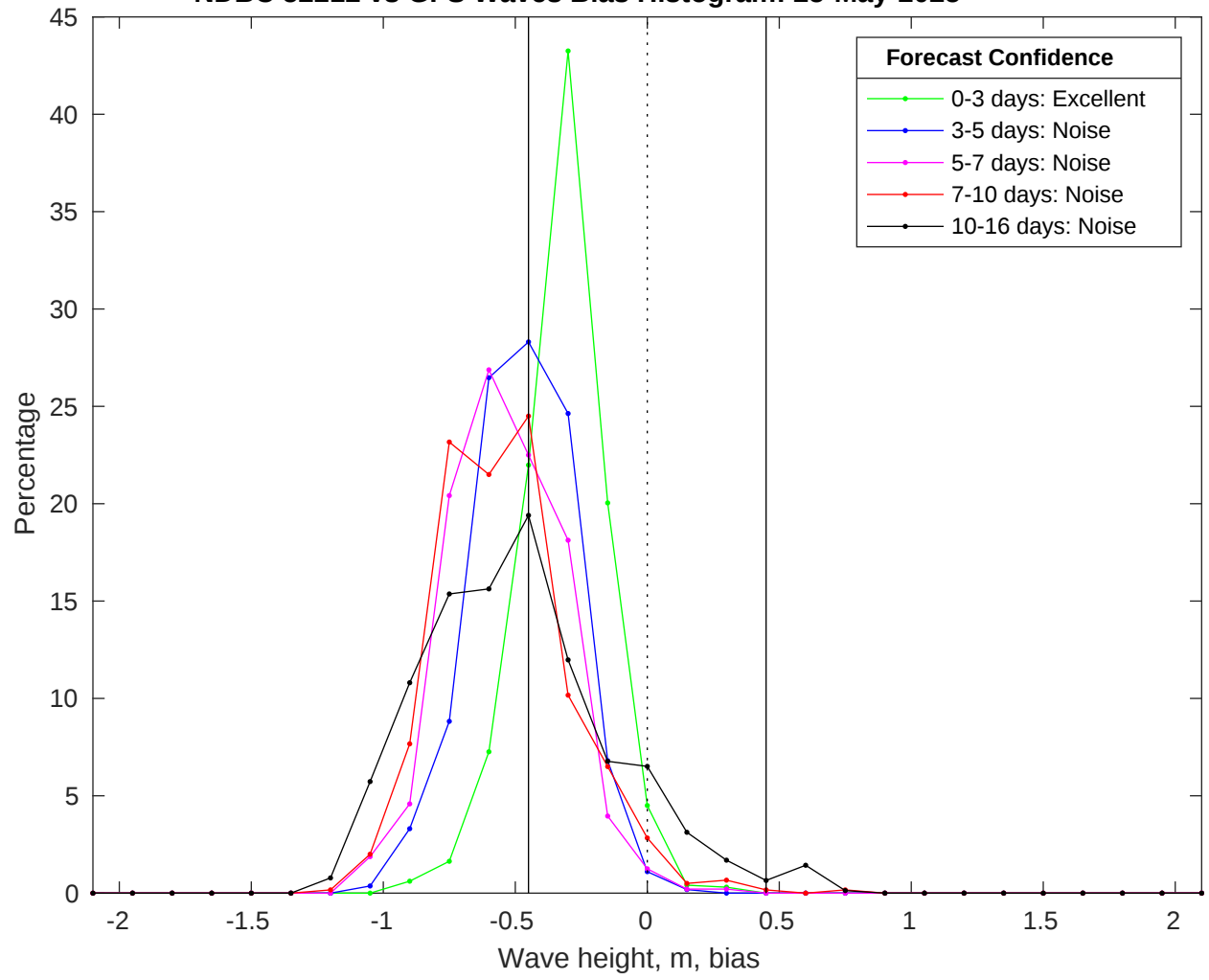
NDBC 52212 vs GFS Waves Bias Histogram: 25-May-2025
