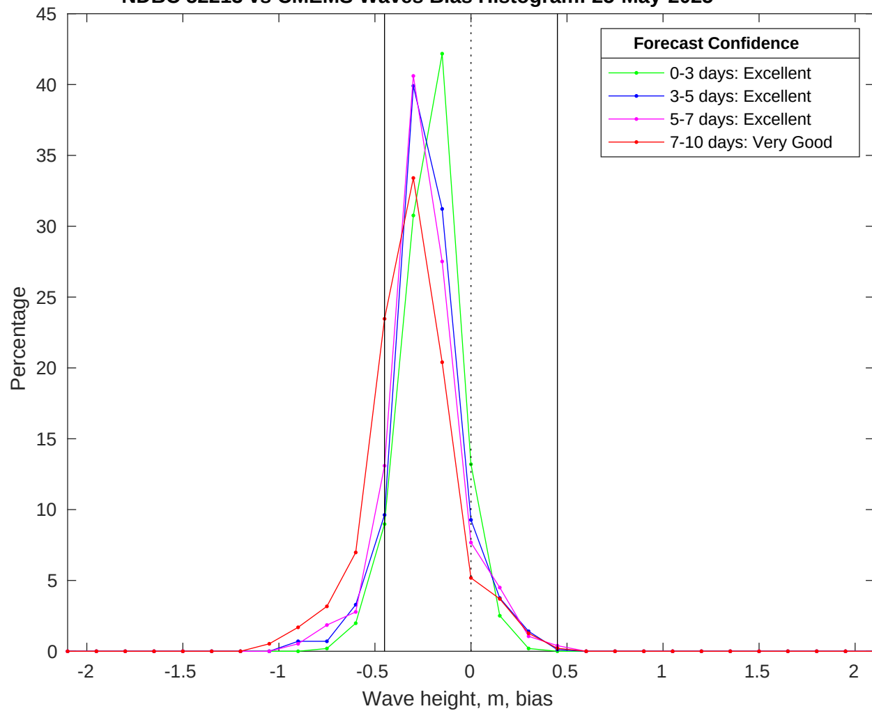
NDBC 52213 vs CMEMS Waves Bias Histogram: 25-May-2025
