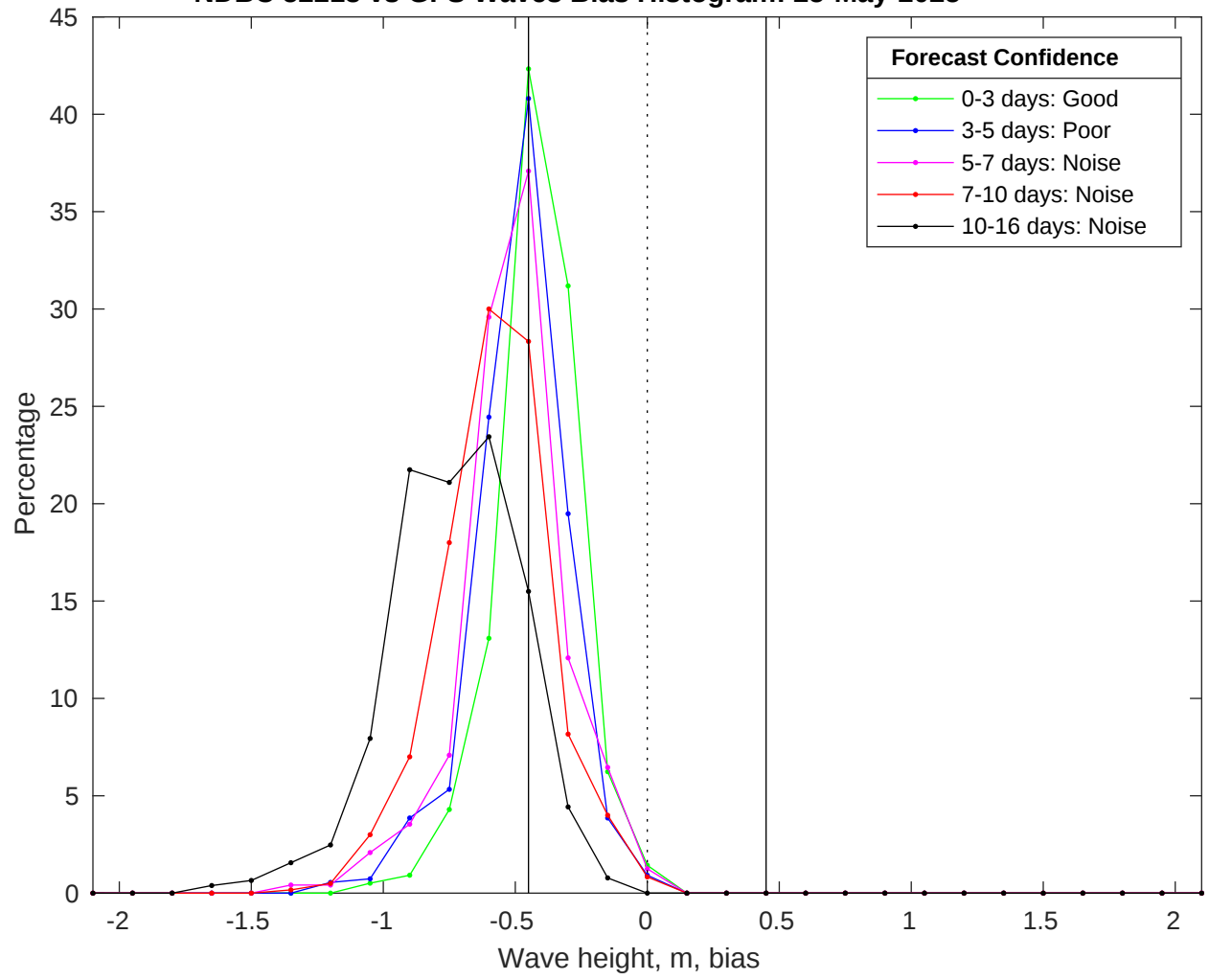
NDBC 52213 vs GFS Waves Bias Histogram: 25-May-2025
