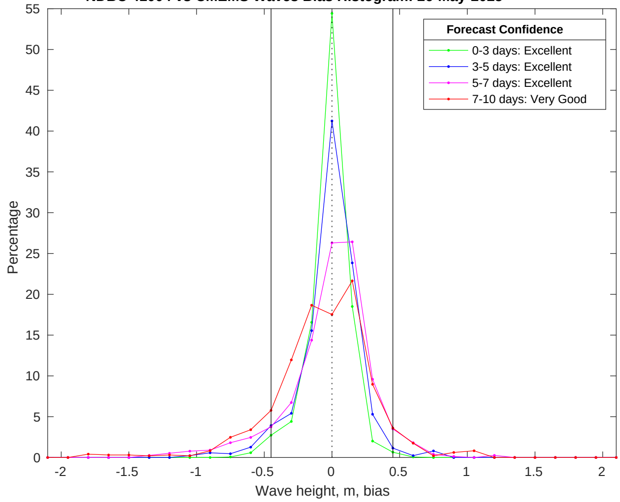
NDBC 41004 vs CMEMS Waves Bias Histogram: 26-May-2025
