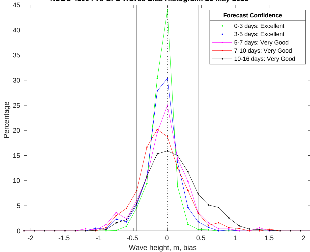
NDBC 41004 vs GFS Waves Bias Histogram: 26-May-2025
