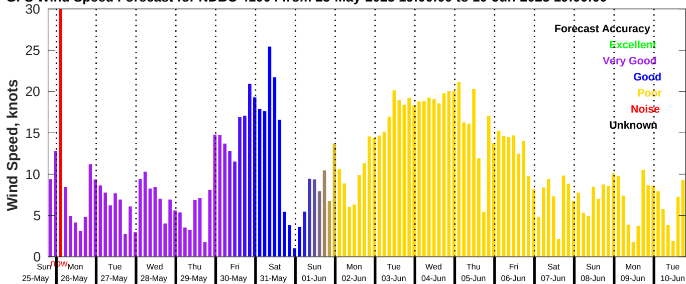
GFS Wind Speed Forecast for NDBC 41004 from 25-May-2025 19:00:00 to 10-Jun-2025 19:00:00
