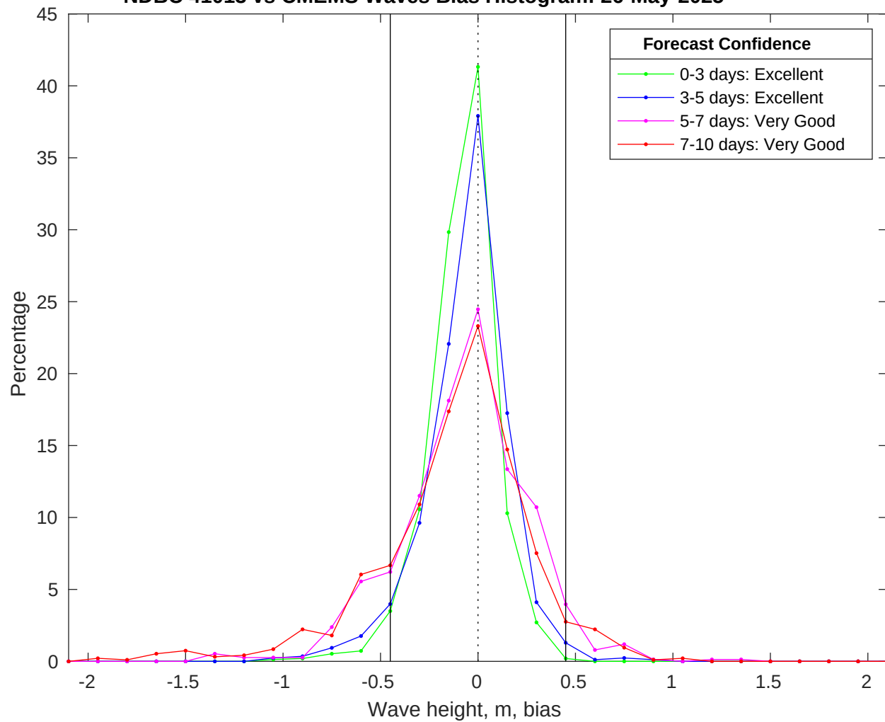
NDBC 41013 vs CMEMS Waves Bias Histogram: 26-May-2025
