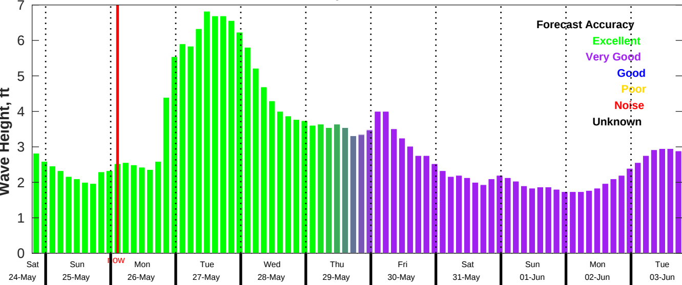
CMEMS Wave Forecast for NDBC 41013 from 24-May-2025 19:00:00 to 03-Jun-2025 19:00:00
