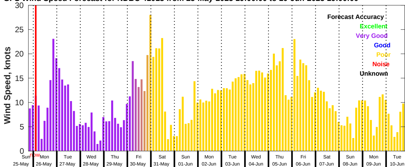
GFS Wind Speed Forecast for NDBC 41013 from 25-May-2025 19:00:00 to 10-Jun-2025 19:00:00
