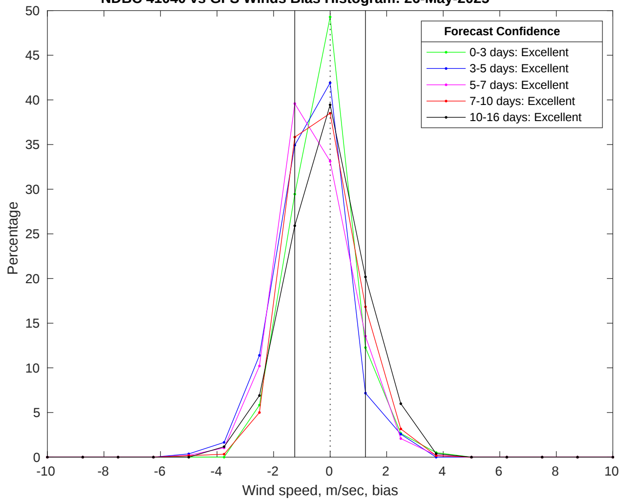
NDBC 41040 vs GFS Winds Bias Histogram: 26-May-2025
