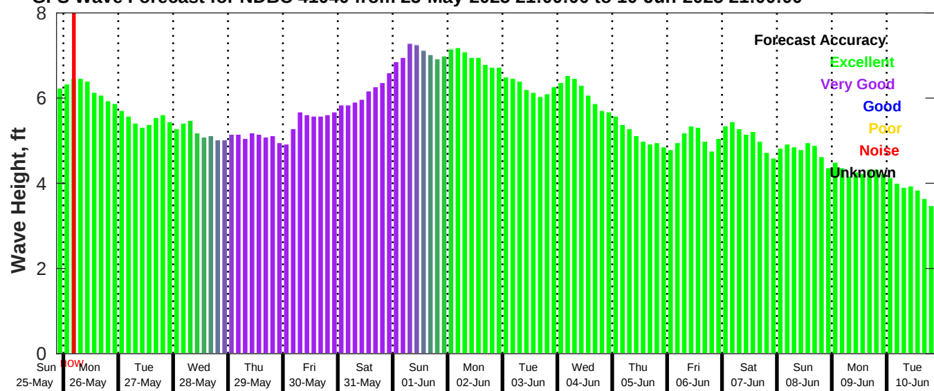
GFS Wave Forecast for NDBC 41040 from 25-May-2025 21:00:00 to 10-Jun-2025 21:00:00
