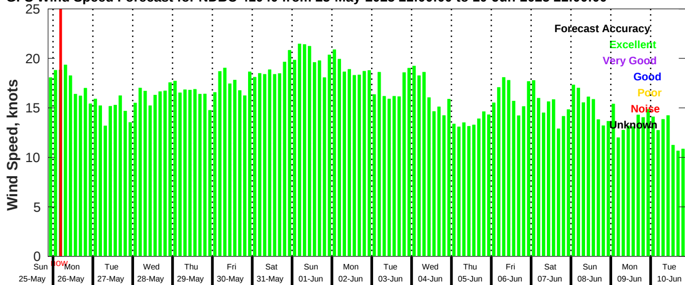
GFS Wind Speed Forecast for NDBC 41040 from 25-May-2025 21:00:00 to 10-Jun-2025 21:00:00
