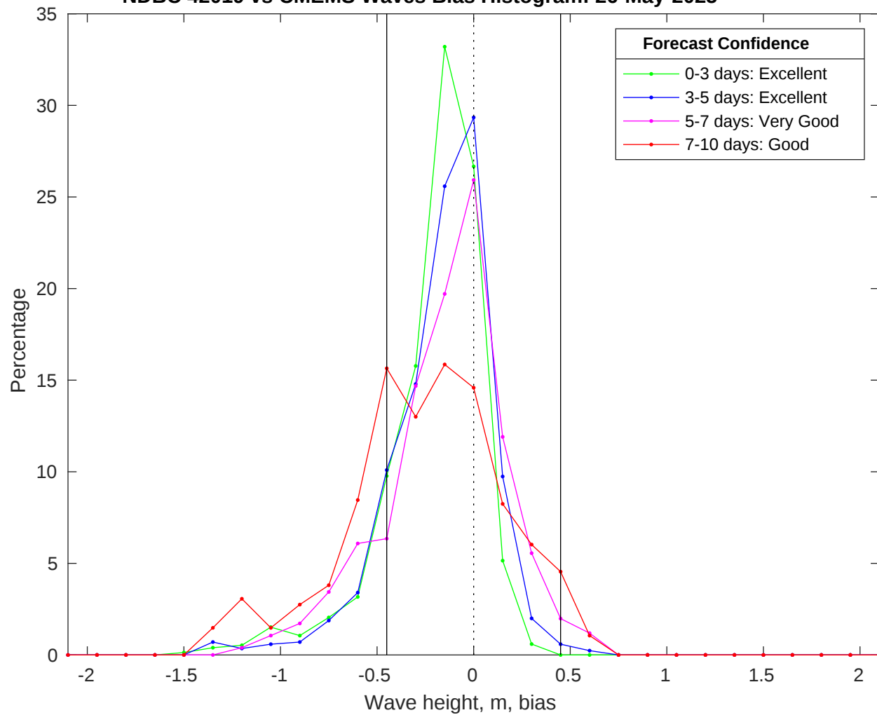
NDBC 42019 vs CMEMS Waves Bias Histogram: 26-May-2025
