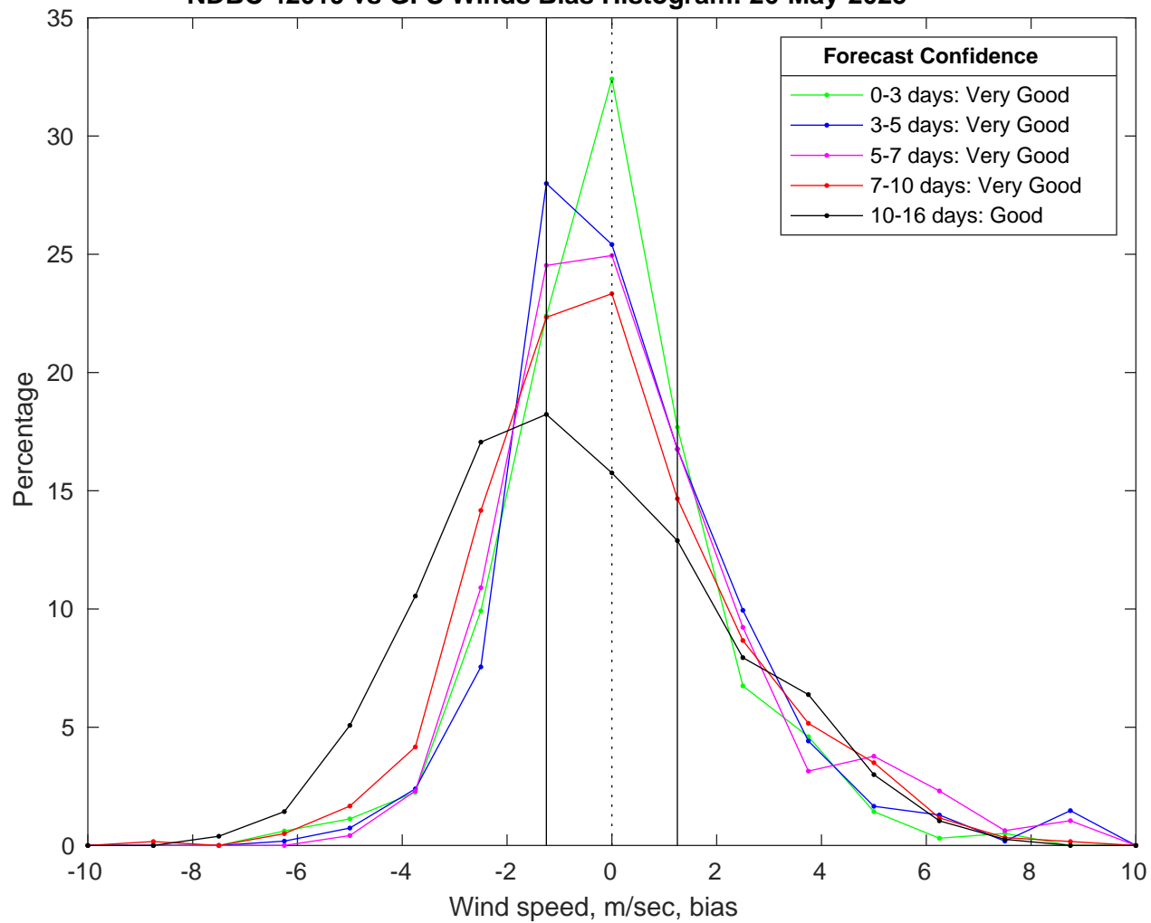
NDBC 42019 vs GFS Winds Bias Histogram: 26-May-2025
