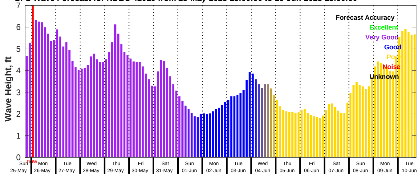
GFS Wave Forecast for NDBC 42019 from 25-May-2025 18:00:00 to 10-Jun-2025 18:00:00
