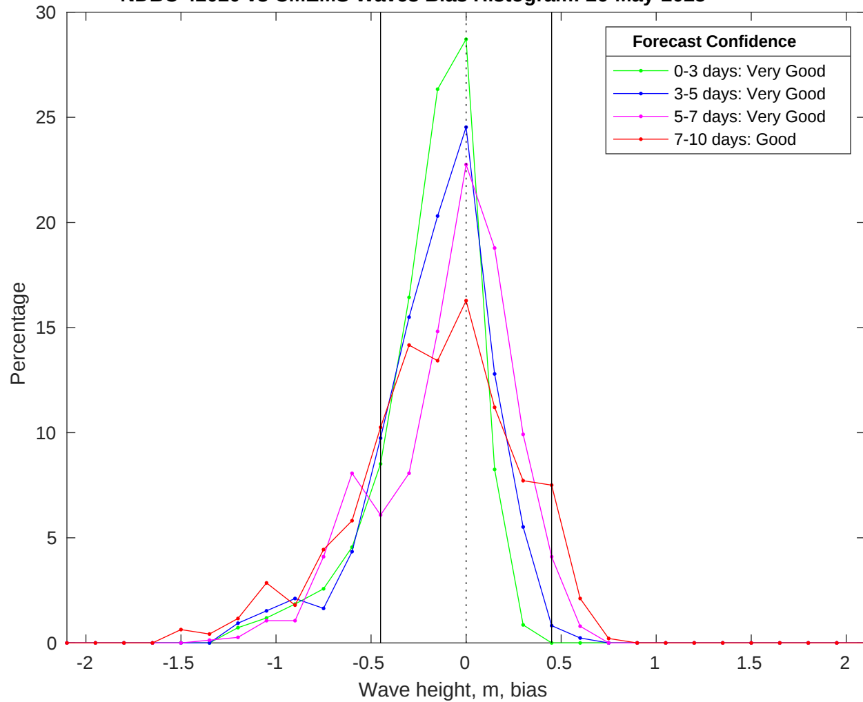
NDBC 42020 vs CMEMS Waves Bias Histogram: 26-May-2025
