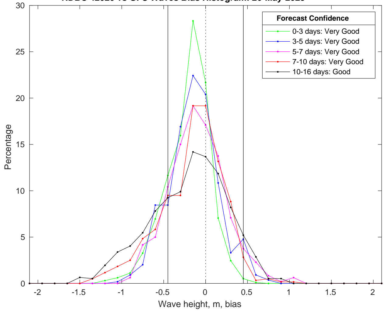
NDBC 42020 vs GFS Waves Bias Histogram: 26-May-2025
