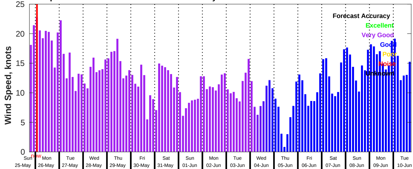
GFS Wind Speed Forecast for NDBC 42020 from 25-May-2025 18:00:00 to 10-Jun-2025 18:00:00
