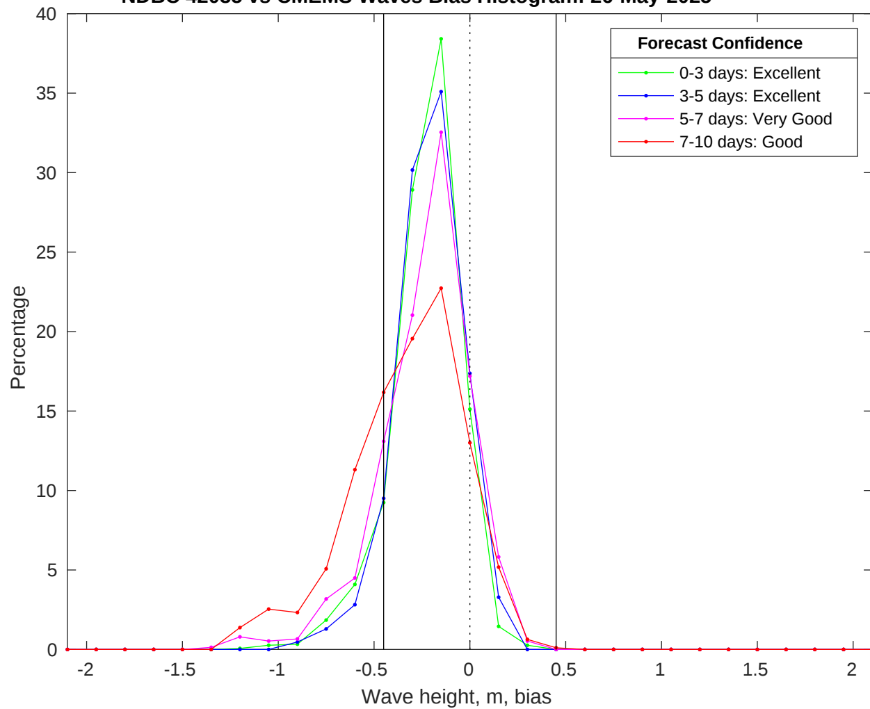
NDBC 42035 vs CMEMS Waves Bias Histogram: 26-May-2025
