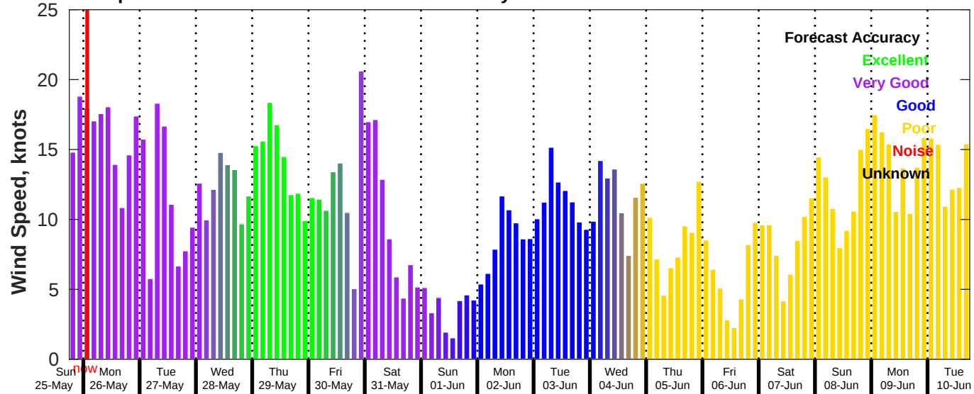
GFS Wind Speed Forecast for NDBC 42035 from 25-May-2025 18:00:00 to 10-Jun-2025 18:00:00
