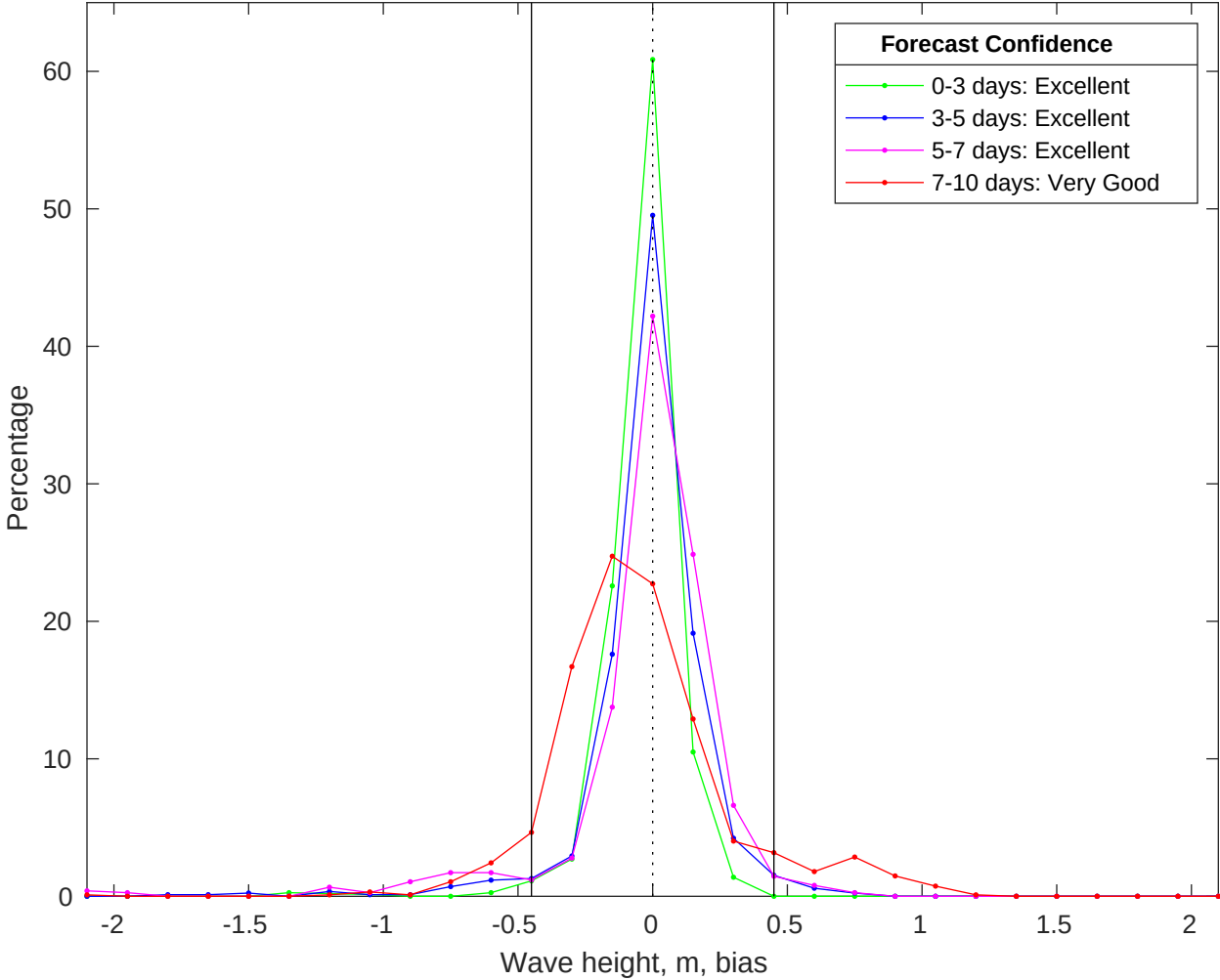
NDBC 42036 vs CMEMS Waves Bias Histogram: 26-May-2025
