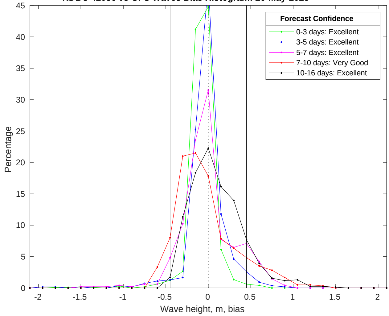
NDBC 42036 vs GFS Waves Bias Histogram: 26-May-2025
