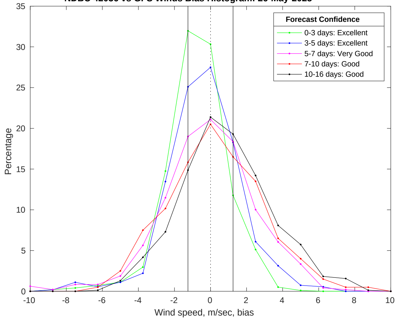
NDBC 42036 vs GFS Winds Bias Histogram: 26-May-2025
