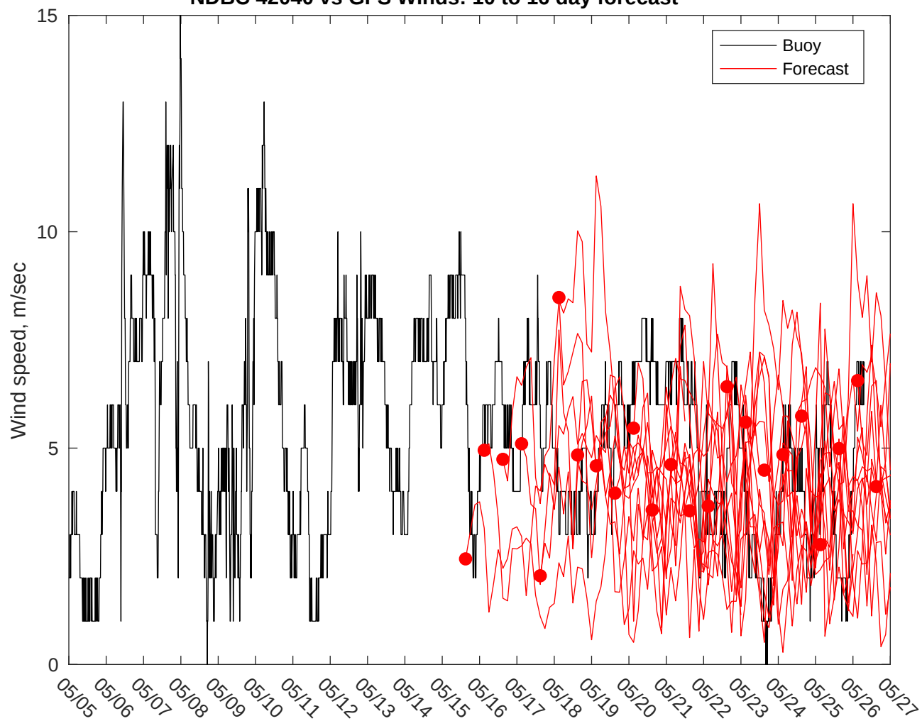
NDBC 42040 vs GFS Winds: 10 to 16 day forecast
