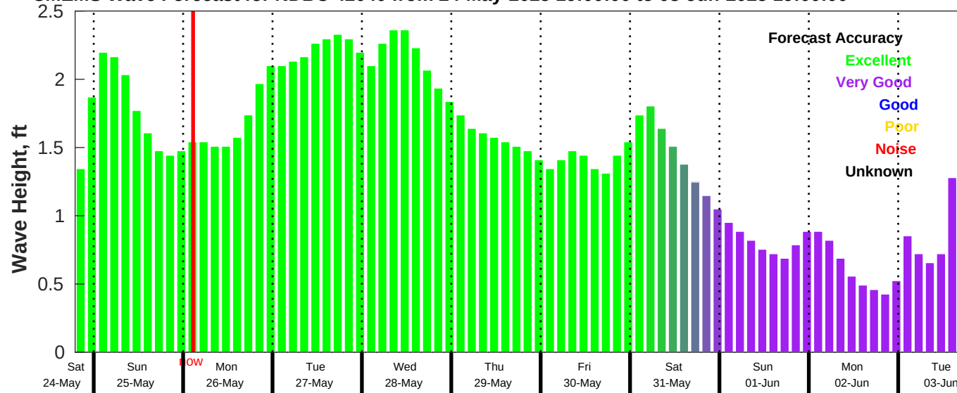
CMEMS Wave Forecast for NDBC 42040 from 24-May-2025 19:00:00 to 03-Jun-2025 19:00:00
