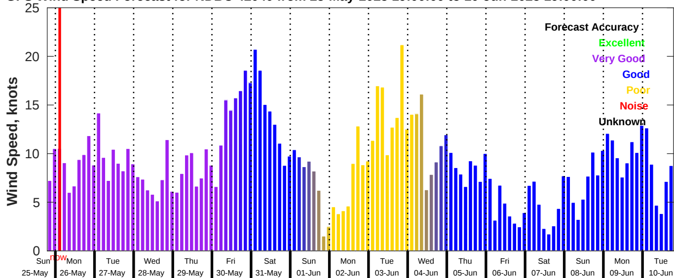
GFS Wind Speed Forecast for NDBC 42040 from 25-May-2025 19:00:00 to 10-Jun-2025 19:00:00
