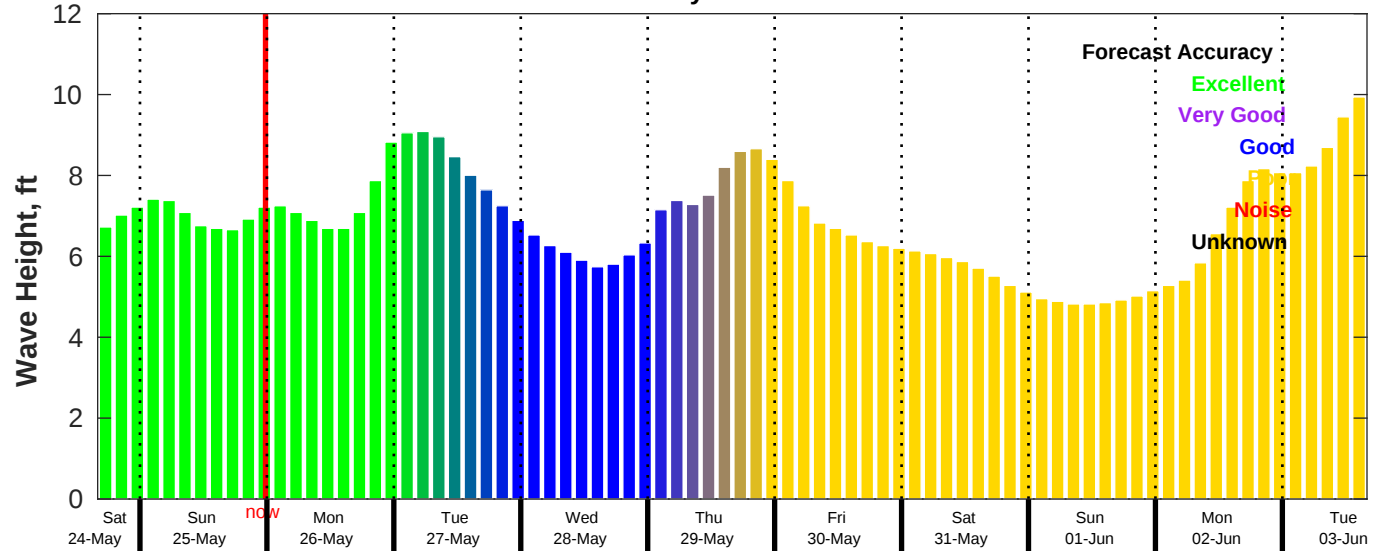
CMEMS Wave Forecast for NDBC 46011 from 24-May-2025 16:00:00 to 03-Jun-2025 16:00:00
