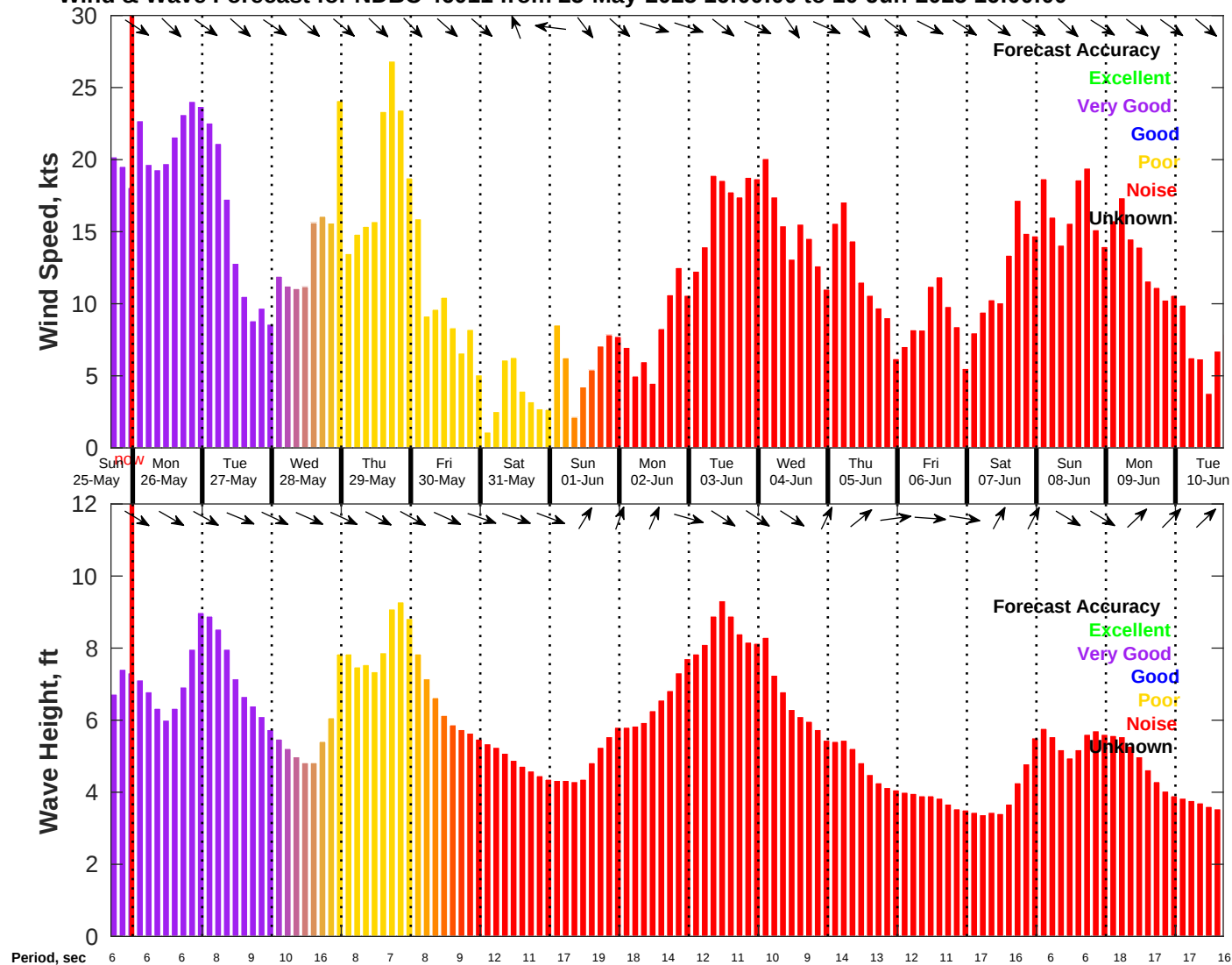
Wind & Wave Forecast for NDBC 46011 from 25-May-2025 16:00:00 to 10-Jun-2025 16:00:00
