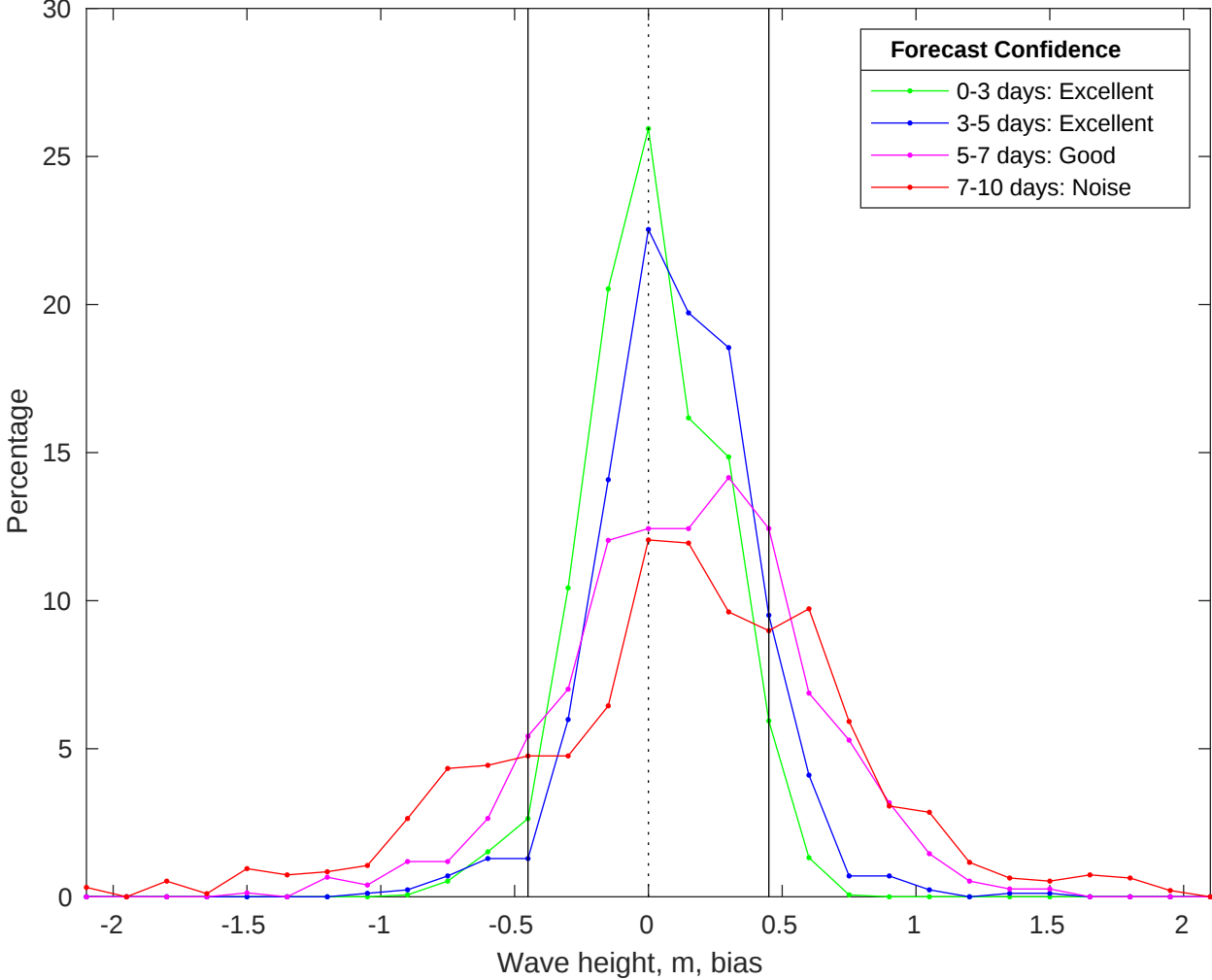
NDBC 46028 vs CMEMS Waves Bias Histogram: 26-May-2025
